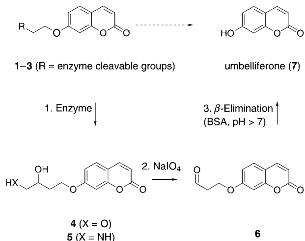
Scheme 1. Principle of periodate-coupled fluorescence assay (see Scheme 2 for R groups).
